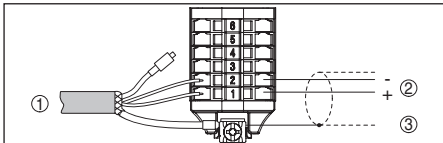
Abb. 26: Schéma de raccordement VEGAWELL S 51 4 ... 20 mA, 4 ... 20 mA/HART
