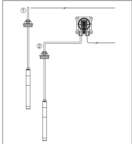
Abb. 15: Connect VEGAWELL S 51 to voltage supply
