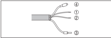
Abb. 16: Wire assignment, suspension cable
