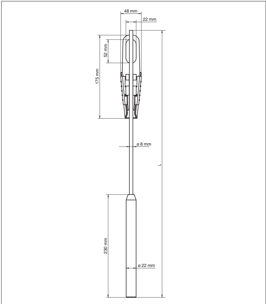
Abb. 18: VEGAWELL S 51
