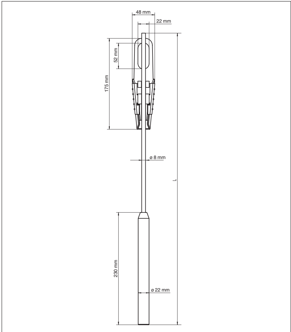
Abb. 27: VEGAWELL S 51
