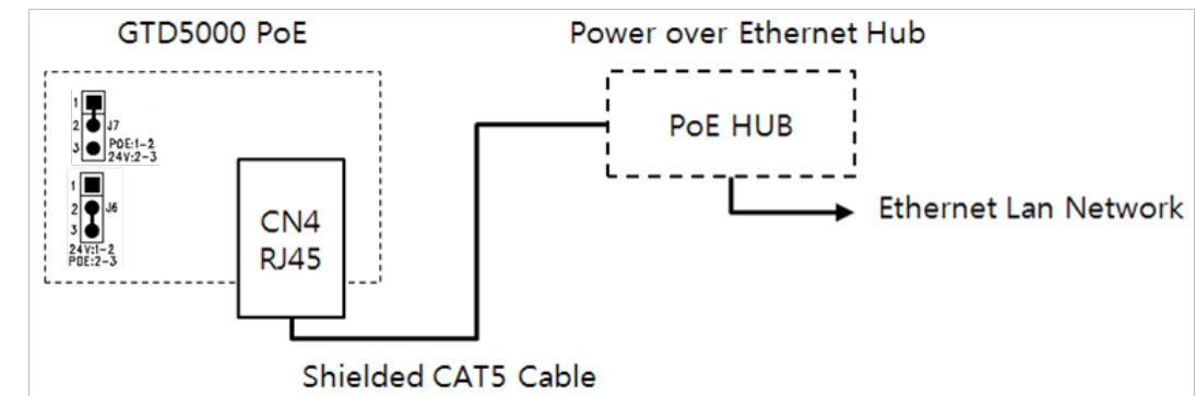
[Figure 11. PoE Configuration]
